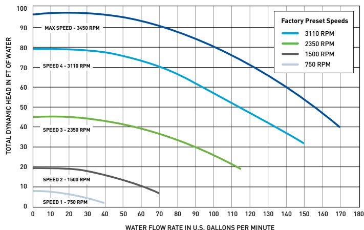
NOTE: The chart above demonstrates performance rates at factory preset speeds of 750 RPM, 1500 RPM, 2350 RPM and 3110 RPM.
